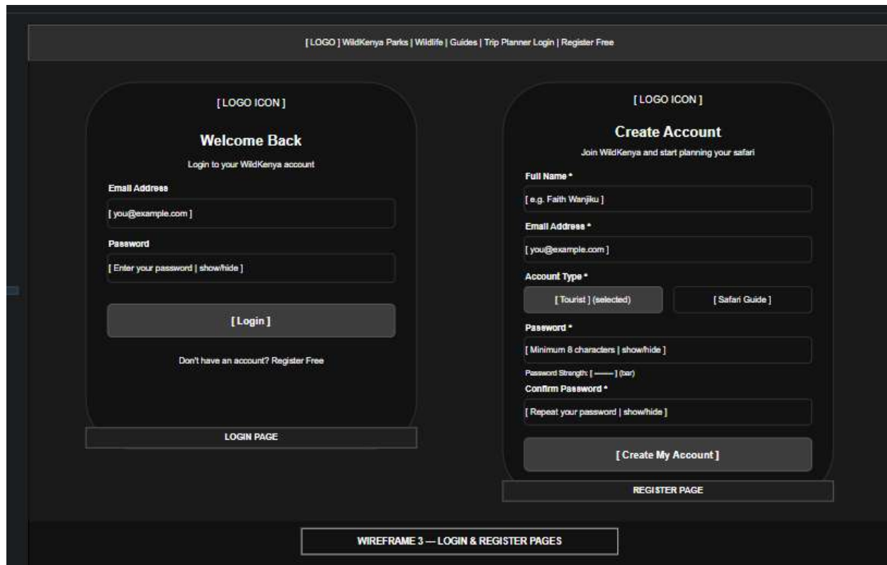
Fig 5: Login and register page wireframes showing form layouts side by side
