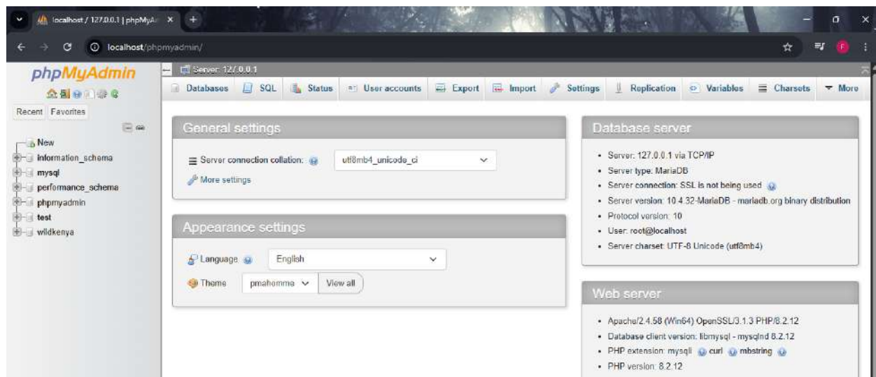
Fig 3-Browser at http://localhost
