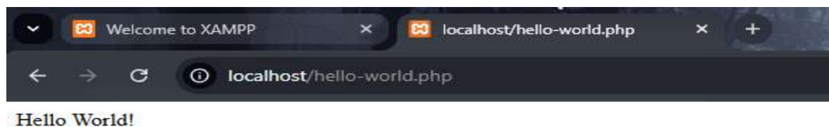
Fig 3-Browser at http://localhost
