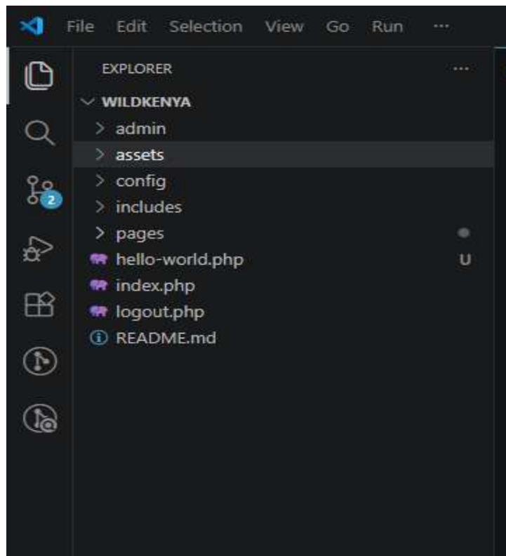
Fig 4-project folder structure
